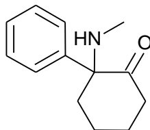
2-(methylamino)-2-phenylcyclohexanone
