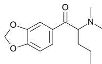
1-(1,3-benzodioxol-5-yl)-2-(dimethylamino)pentan-1-one
